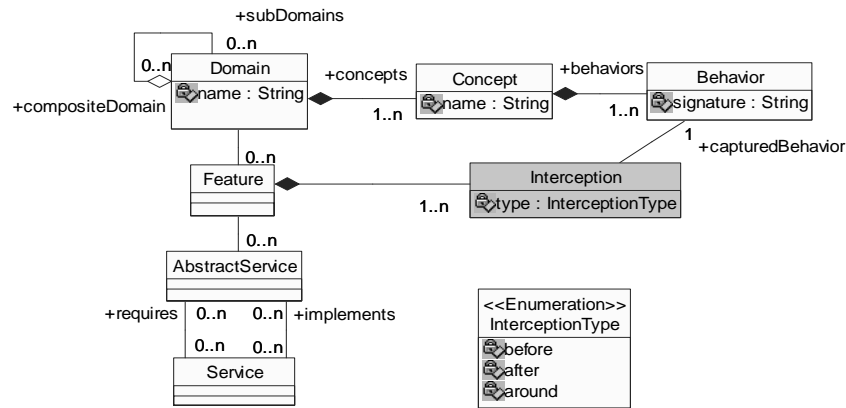
Fig. 4. Metamodel for the vertical composition
