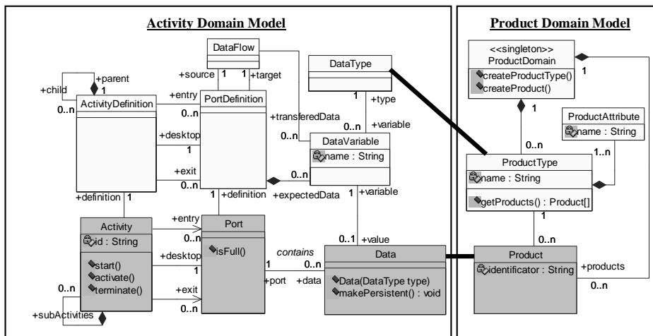
Fig. 2. Activity domain model vs. Product domain model
