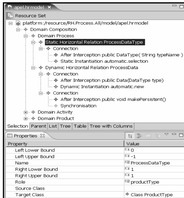
Fig. 6. Defining horizontal relationships at metamodel level.
