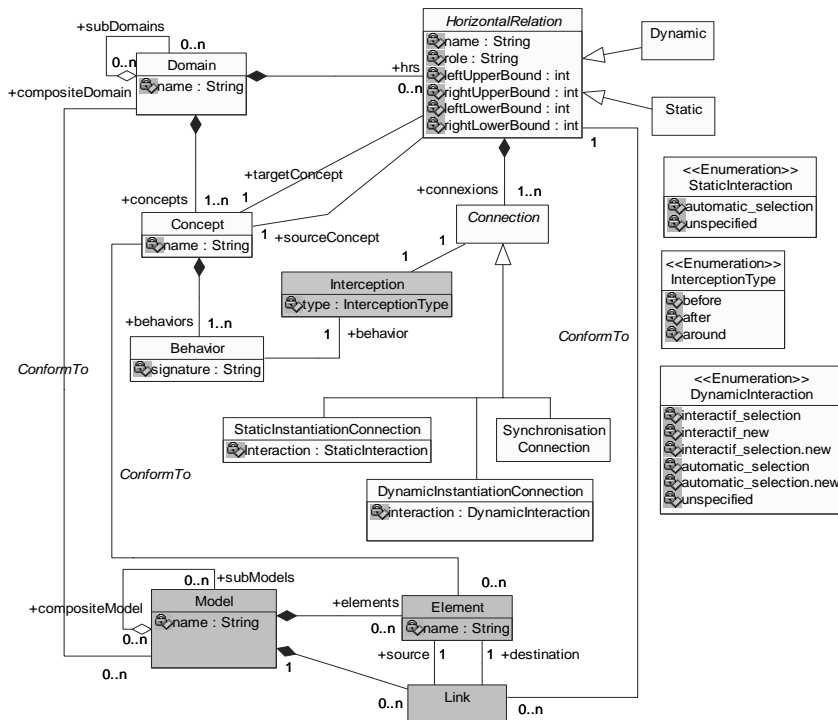
Fig. 5. Metamodel for the horizontal composition
