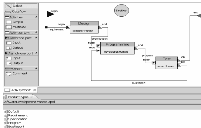
Fig. 3. An Activity model (fragment)
