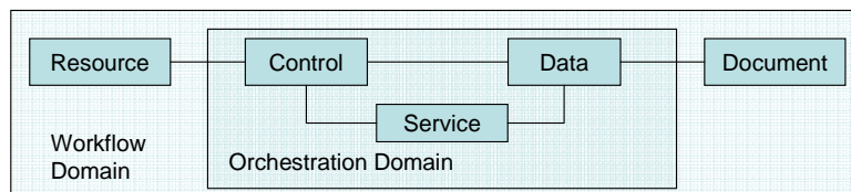
Fig. 8 Workflow Domain
